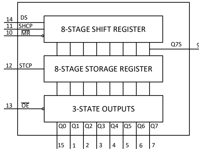
Fig. 1. Functional diagram
