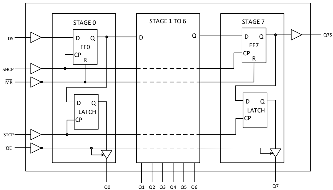
Fig. 4. Logic diagram
