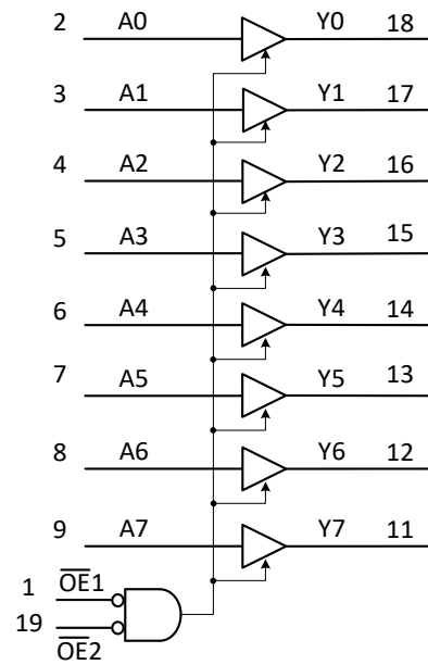
Fig. 2. Functional diagram
