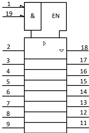
Fig. 1. IEC logic symbol
